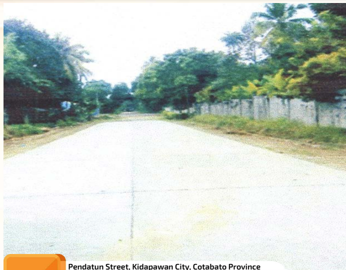
Project Cost: 1,238,577.99 Pendatun Street, Kidapawan City, Cotabato Province Road Concreting 55 Linear Meter - 2 lane Road Concreting
