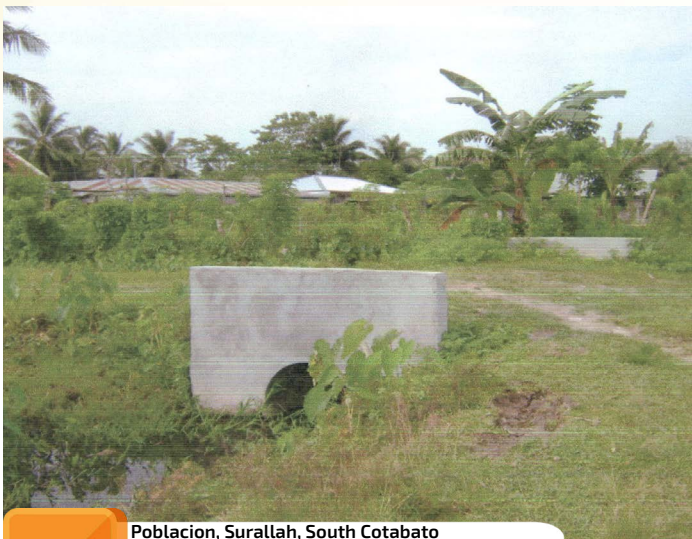
Project Cost: 1,075,540.00 Poblacion, Surallah, South Cotabato Fabrication and Installation of RC Pipes Phase I & II)
