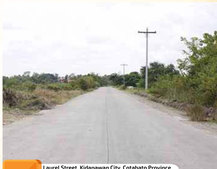
Project Cost: 1,855,885.40 Laurel Street, Kidapawan City, Cotabato Province Concreting of City Roads Concreting of City Roads 2 lane pavement Width 6.7 M, Thick .20M wd a length of 468 ln m. Provision of 2 line -48" dia. RCCP & 1 line -36" dia. RCCP
